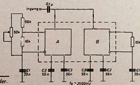
Fig. 8. Hystereseschakeling.
